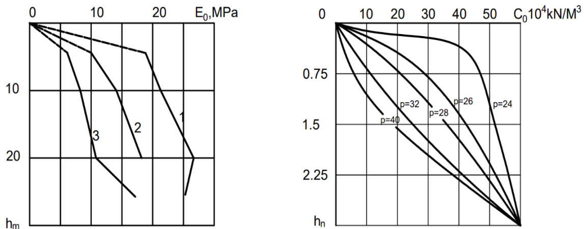
Figure 2. Variation of the modulus of subsidence with depth (a) and the stiffness of the supports under the action of loads C(x_k) coefficients. 1,2,3 - natural, partially and completely desalinated soil conditions, respectively (pile length 3.0m, cross-section 20x20cm) (Central Fergana).
